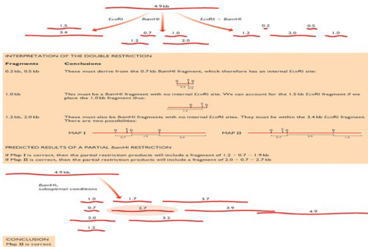
Figure 4. The objective is to map the EcoRI (E) and BamHI (B) sites in a linear DNA molecule of 4.9kb
